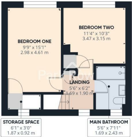
Floor 1 Building 1
